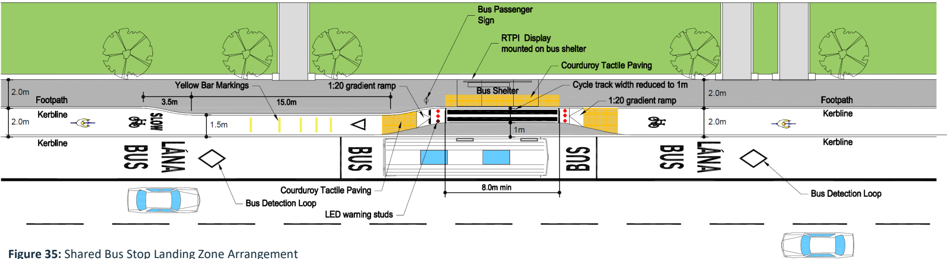
Figure 35: Shared Bus Stop Landing Zone Arrangement
