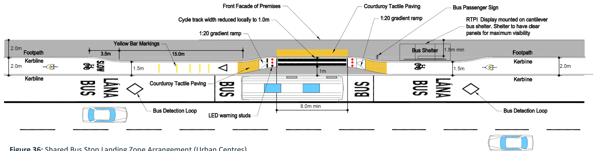
Figure 36: Shared Bus Stop Landing Zone Arrangement (Urban Centres)
