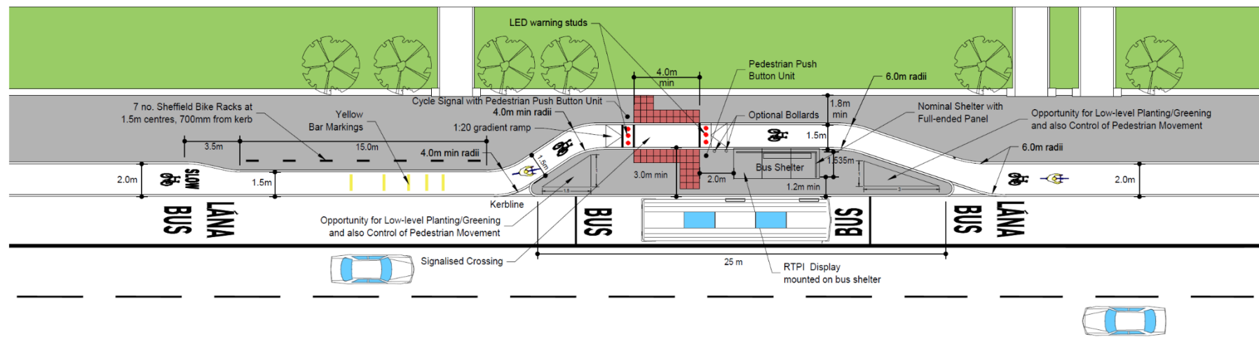
Figure 34: Island Bus Stop Arrangement
