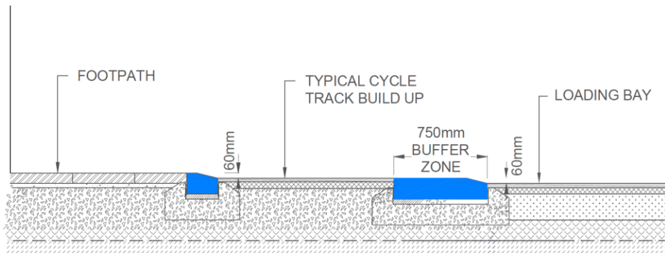
Figure 13a: Proposed Loading Bay Cross Section with Chamfered Kerbs
