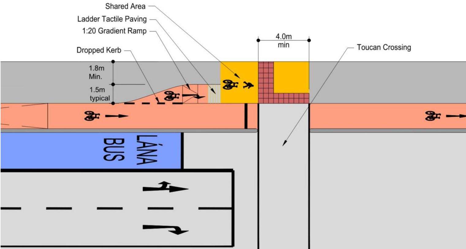
Figure 28: Preferred Cyclist Waiting Area Detail at Toucan crossing
