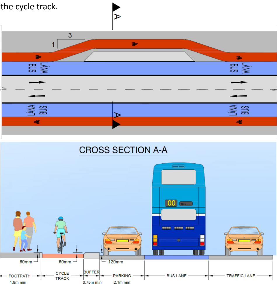
Figure 12: Parking protected cycle track
