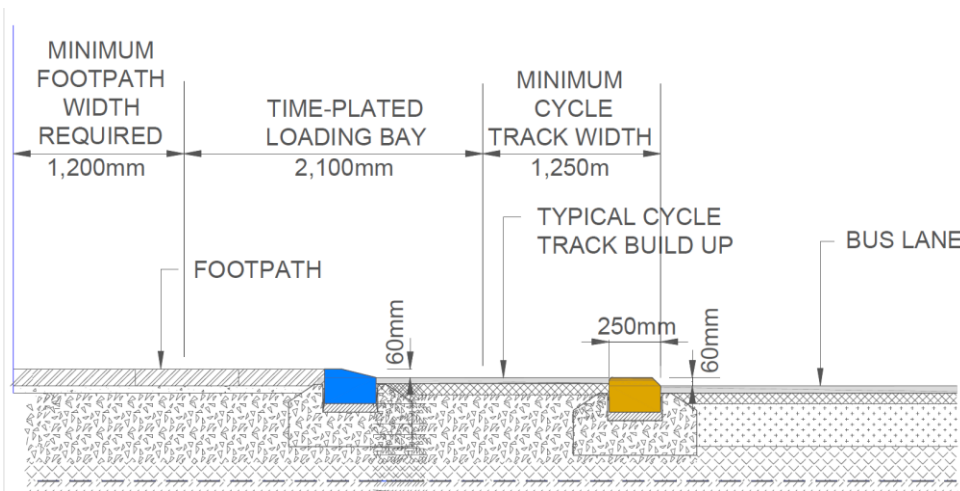
Figure 13b: Loading Bay in confined location that straddles both cycle track and footpath
